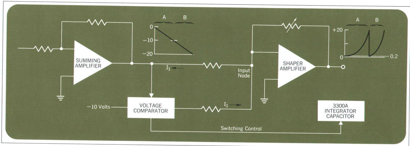
Fig. 6. The two exponential curves at the right are generated from the single ramp at the left. As the ramp voltage goes from 0 to -10, current is drawn from the shaper amplifier causing its output to rise exponentially from 0.2 to 20 volts. At -10 volts on the ramp, the voltage comparator switches the precise amount of current being drawn. This causes the shaper amplifier to reset to 0.2 volt. The voltage comparator continues to supply current as the ramp proceeds from -10 to -20 volts, resulting in the second exponential B, at the right.
